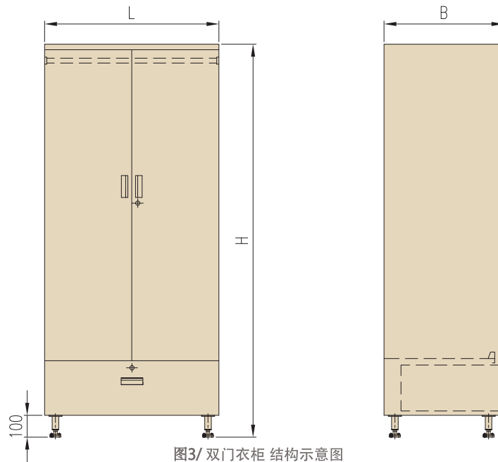
PIC3/ DOUBLE DOOR WARDROBE STRUCTURE DIAGRAM
